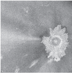
Venus - Adivar Crater
