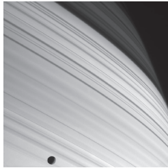
Sun-striped Saturn
