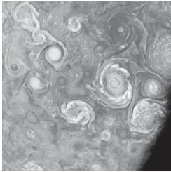
Vortices Near Jupiter's North Pole
