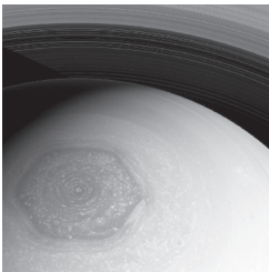
Saturn Polar Jet
