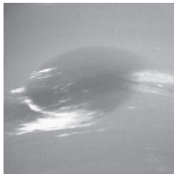
Neptune Great Dark Spot
